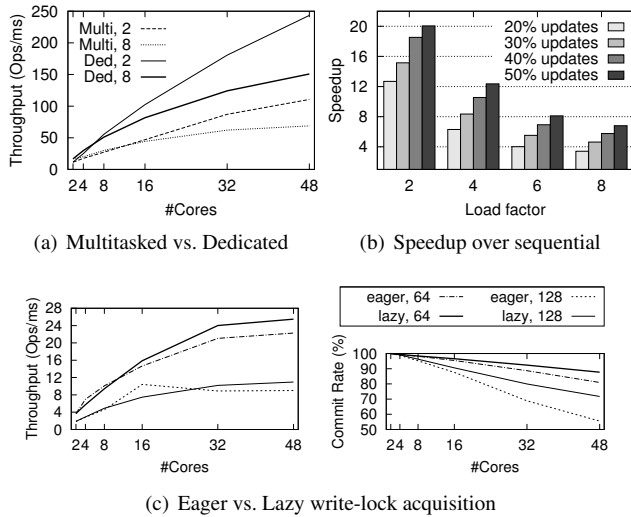
Figure 4. The hash table benchmark
