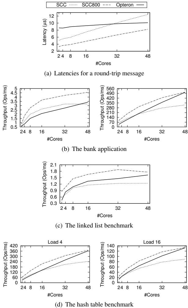
Figure 8. TM 2 C performance on many-core (SCC/SCC800) vs. multi-core (Opteron)
