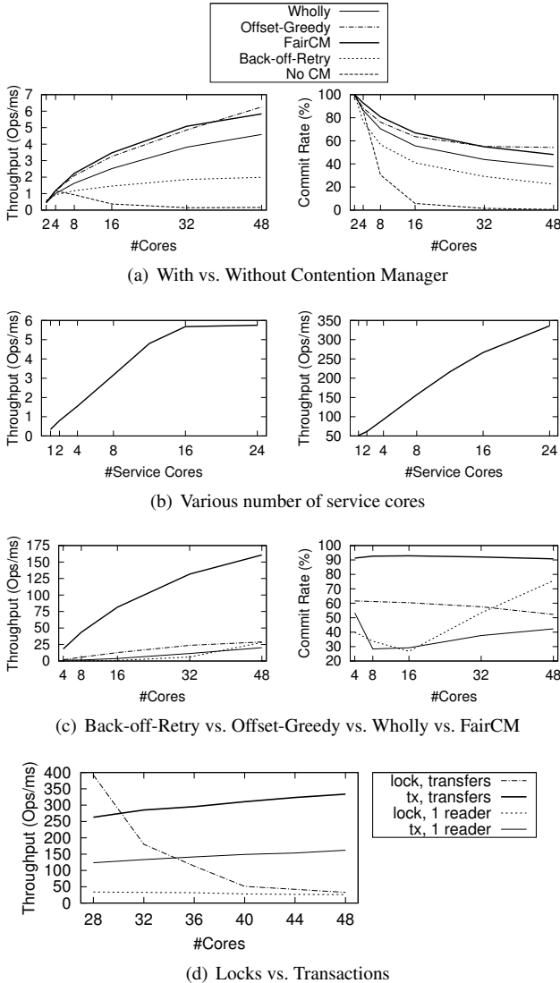
Figure 5. The bank application
